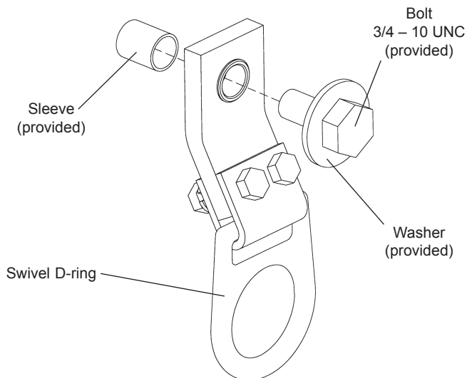
FIGURE 1 INSTALLATION DIAGRAM
