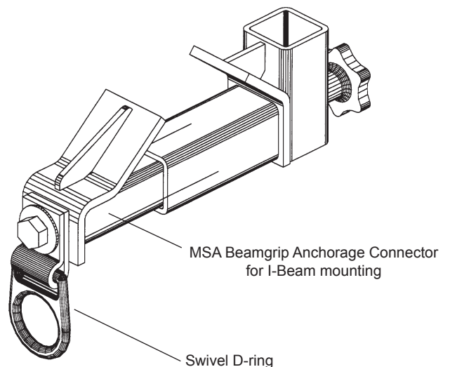
FIGURE 2 COMPLETED ASSEMBLY VIEW
